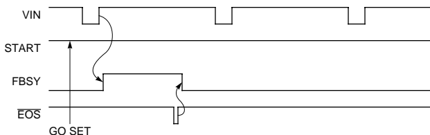
Figure 19. Processing Controlled by GO/STOP Register in Single Frame Compression Mode ( CNT1 = 0 )
