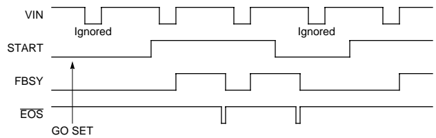
Figure 21. Sequential Mode Operation ( CNT1 = 1 ) with START Control
