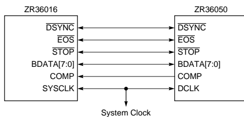
Figure 30. ZR36016 to ZR36050 Connections
