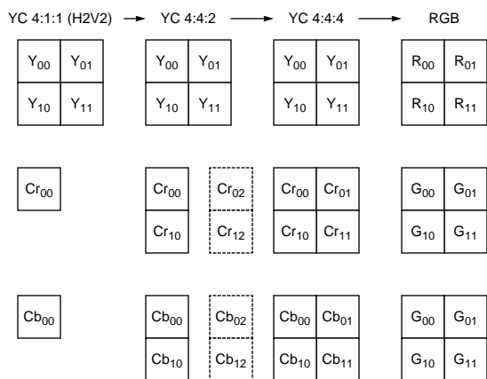
Figure 14. Interpolation Flow
