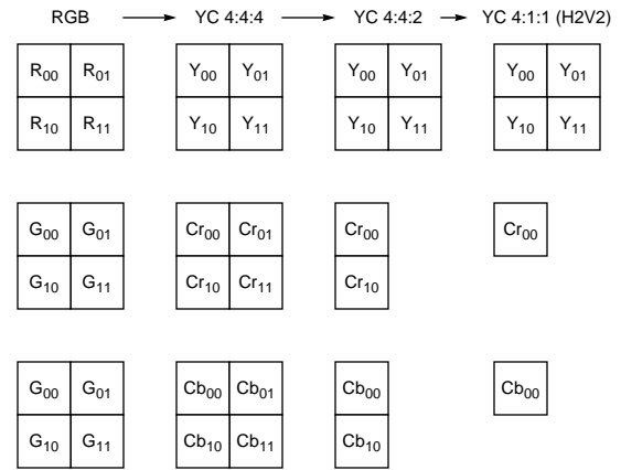
Figure 13. Decimation Flow
