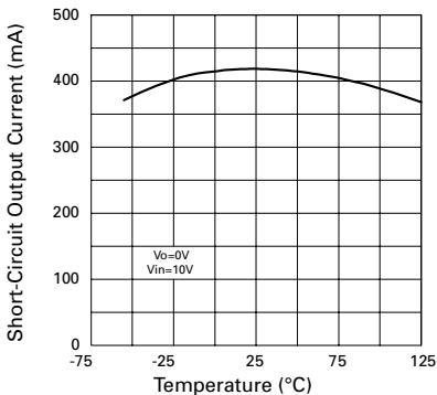
Peak Output Current v Temperature
