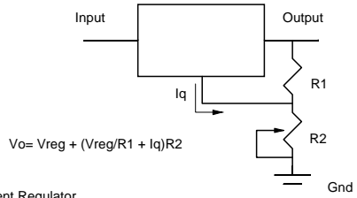
Current Regulator
