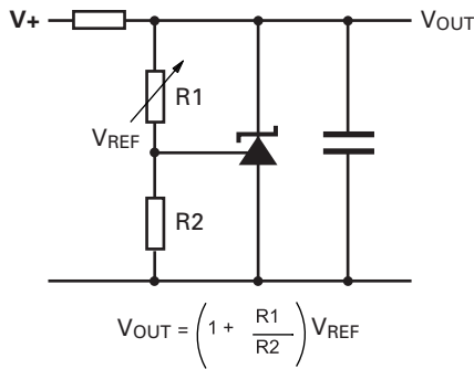
Shunt regulator
