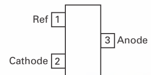
ZTLV431_F (SOT23) (top view)
