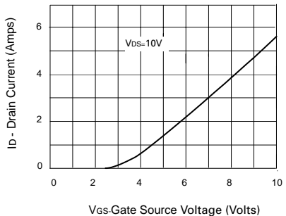
Transfer Characteristics
