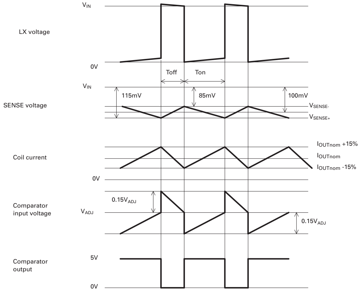
Figure 1 - Operating waveforms
