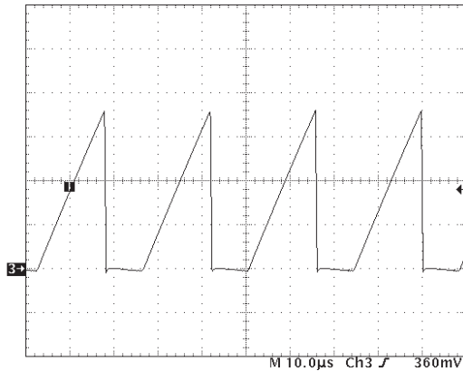
Figure 5. Inductor current (200mA/div)
