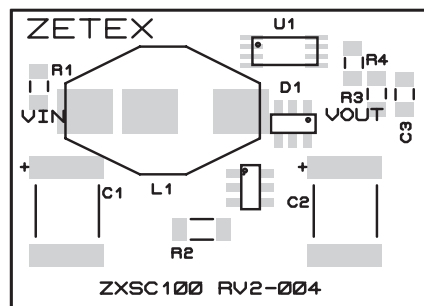
Top silk
