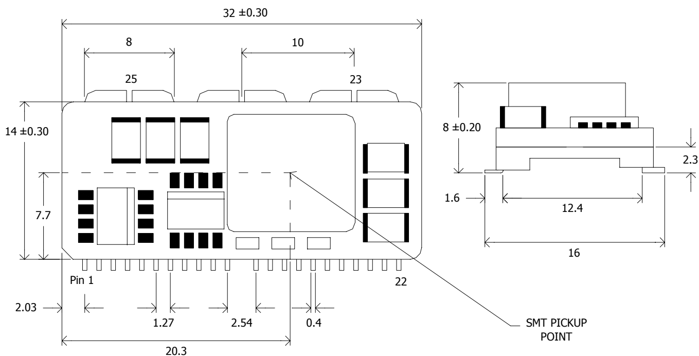
Figure 20. Mechanical Drawing
