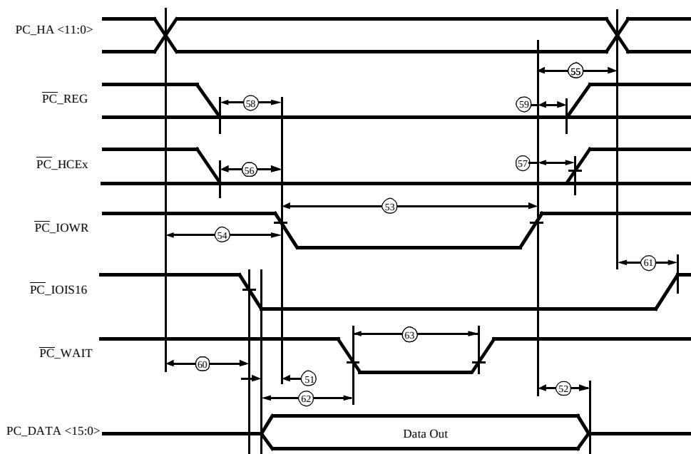
Figure 22. I/O Write Timing
