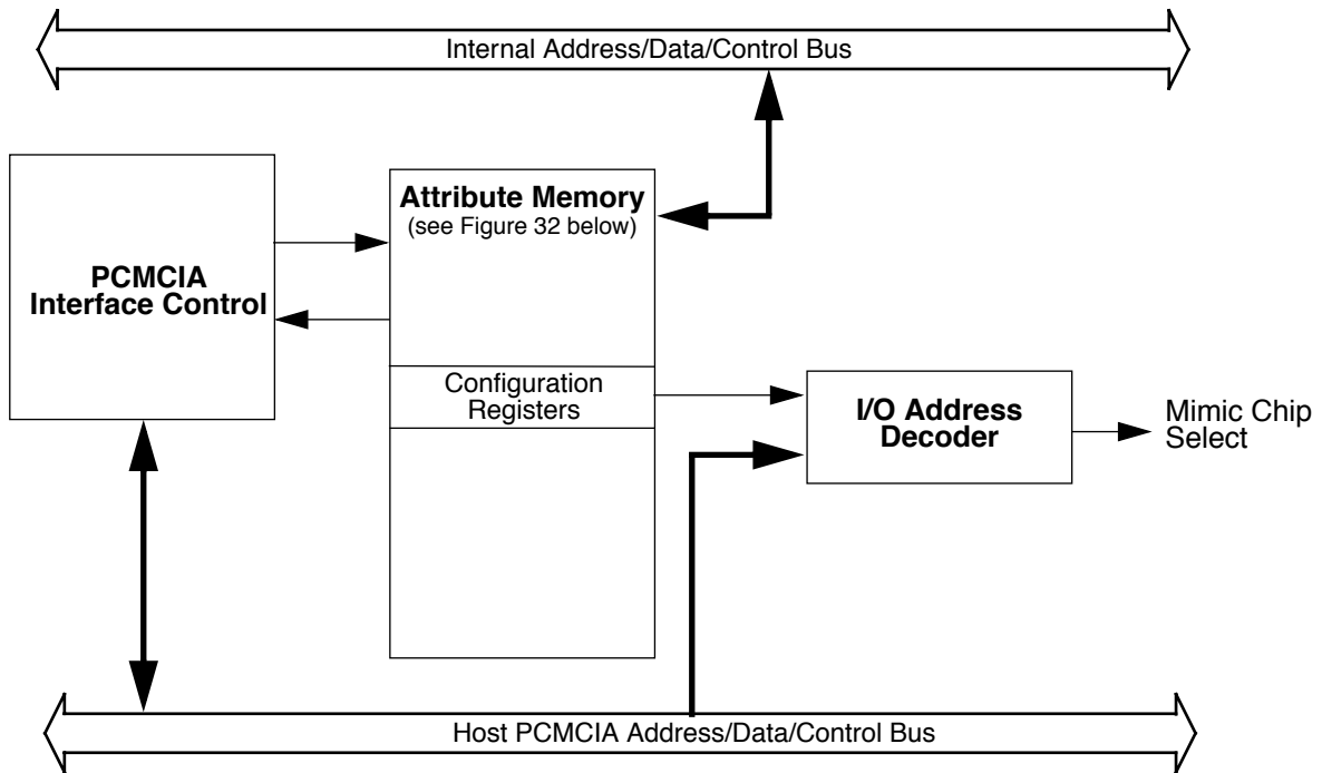
Figure 27. PCMCIA Interface
