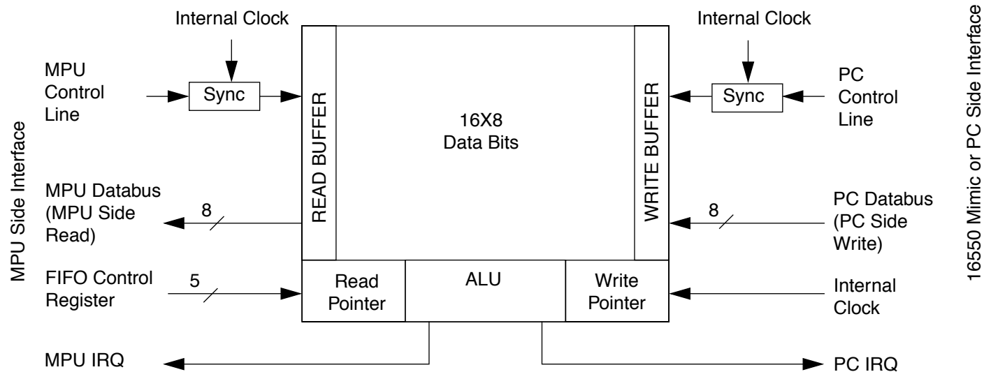
Figure 25. 16550 Mimic Transmitter FIFO Block Diagram
