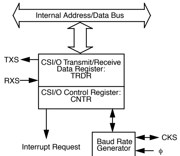
Figure 34. CSI/O Block Diagram
