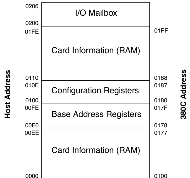
Figure 28. PCMCIA Attribute Memory Organization
