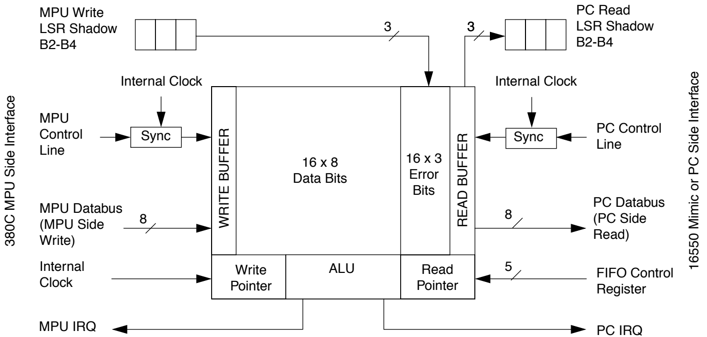
Figure 24. 16550 Mimic Receiver FIFO Block Diagram
