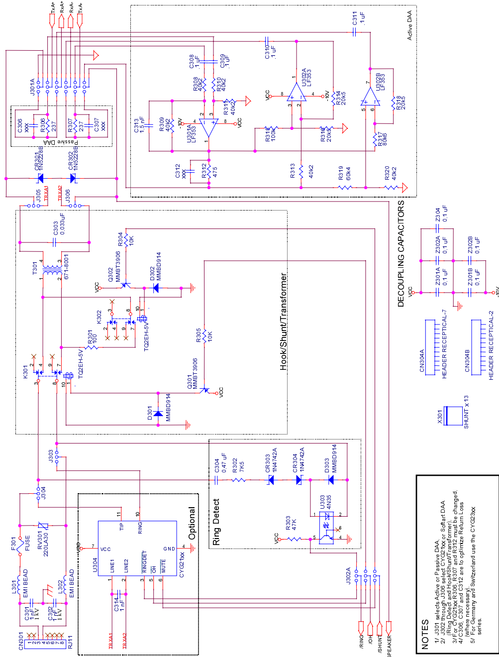
Figure 15. Example DAA
