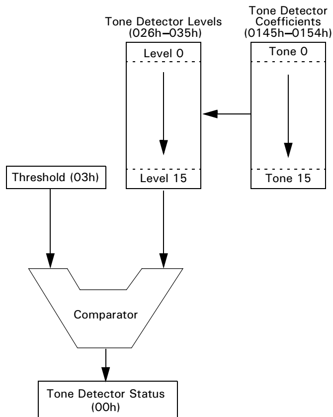
Figure 11. Tone Detectors
