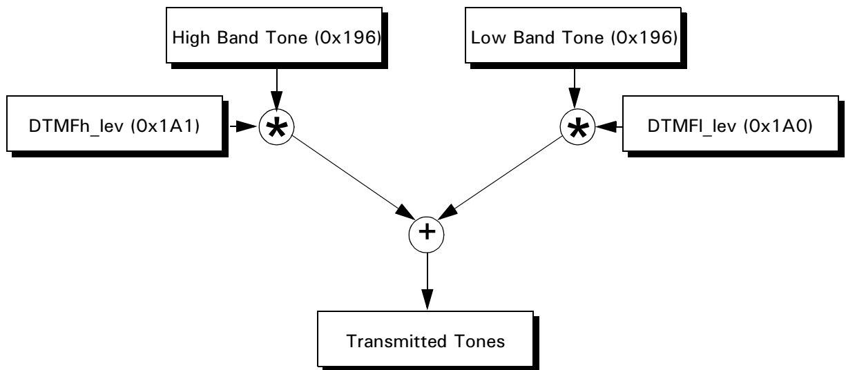
Figure 10. Transmitting Tones
