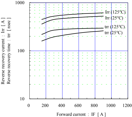
Reverse recovery characteristics (typ.) Vcc=600V, VGE=±15V, Rg=0.6Ω
