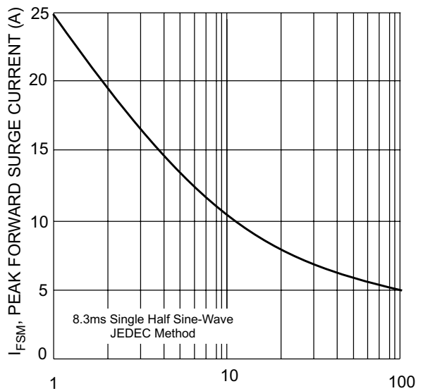
NUMBER OF CYCLES AT 60 Hz Fig. 4, Maximum Non-Repetitive Peak Fwd Surge Current
