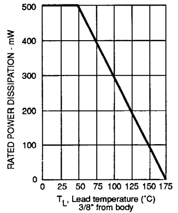
FIGURE 3 POWER DERATING CURVE
