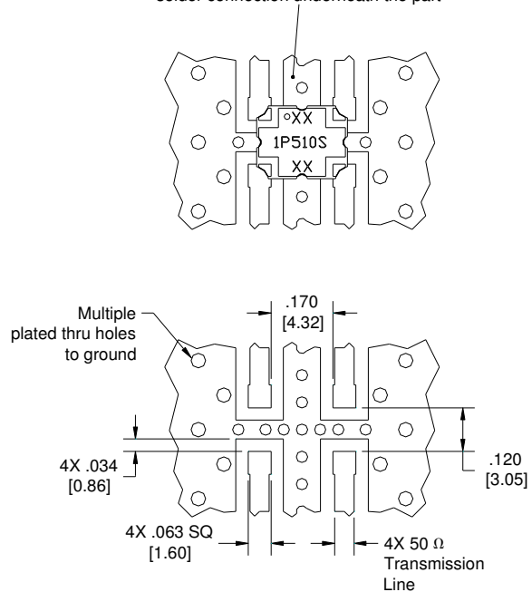
Dimensions are in Inches [Millimeters] 1P510S Mounting Footprint
