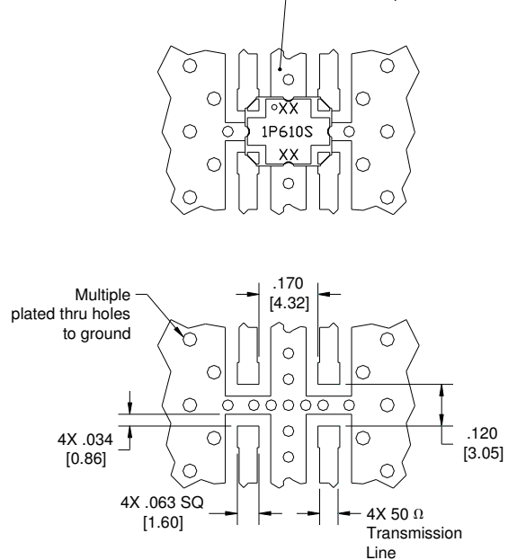
Dimensions are in Inches [Millimeters] 1P610S Rev A Mounting Footprint
