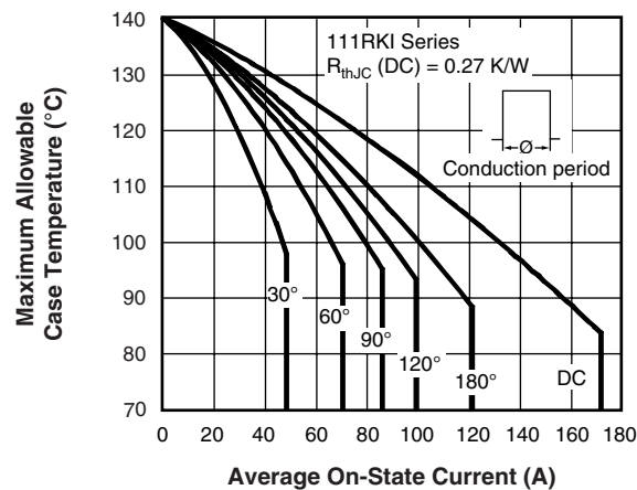
Fig. 2 - Current Ratings Characteristics
