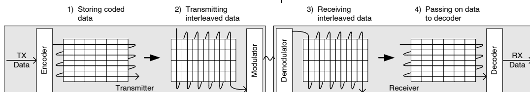
Figure 9: General principle of matrix interleaving
