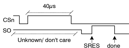
Figure 11: Power-up with SRES
