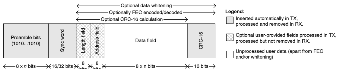
Figure 8: Packet Format
