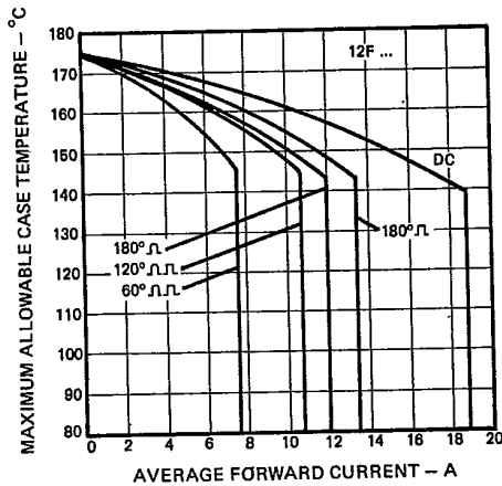
Fig. 8 - Average Forward Current Vs. Maximum Allowable Case Temperature, 12F Series Note: add 2°C to above curves at full rated load for 12F-B series.
