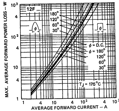
Fig. 9 - Maximum Forward Power Loss Vs. Average Forward Current, 12F Series Note: subtract 3 percent from above curves at full rated load for 12F-B series.
