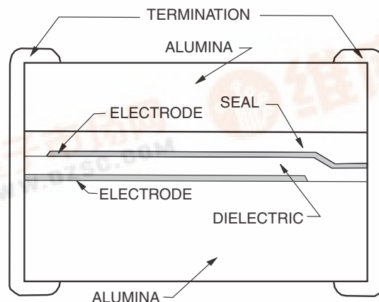
ACCU-P® CAPACITOR
