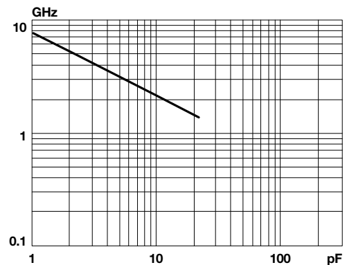
Typical Self Resonant Frequency vs. Capacitance Accu-F ® /Accu-P ® 0603
