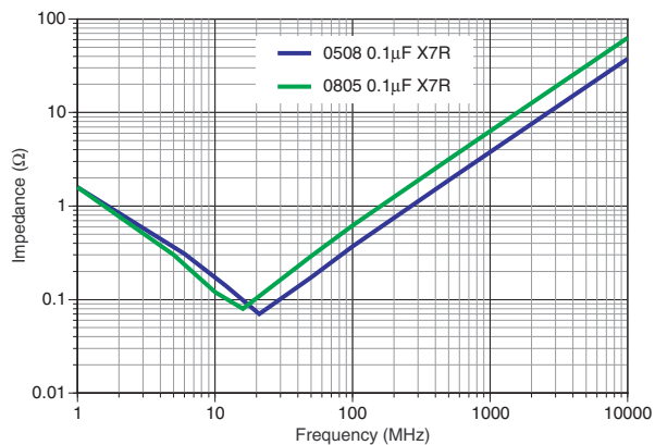
IMPEDANCE 0508 vs. 0805
