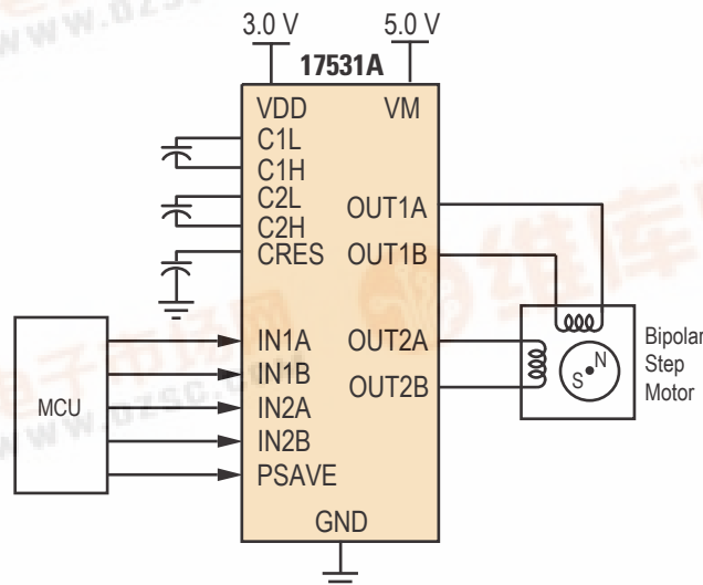
Figure 1. 17531A Simplified Application Diagram
