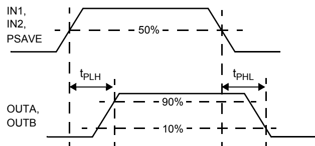
Figure 5. t_{PLH} , t_{PHL} , and t_{PZH} Timing
