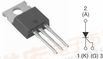
TO-220AB
