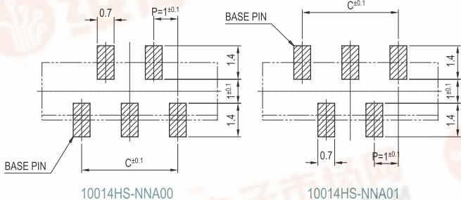
PCB LAYOUT
