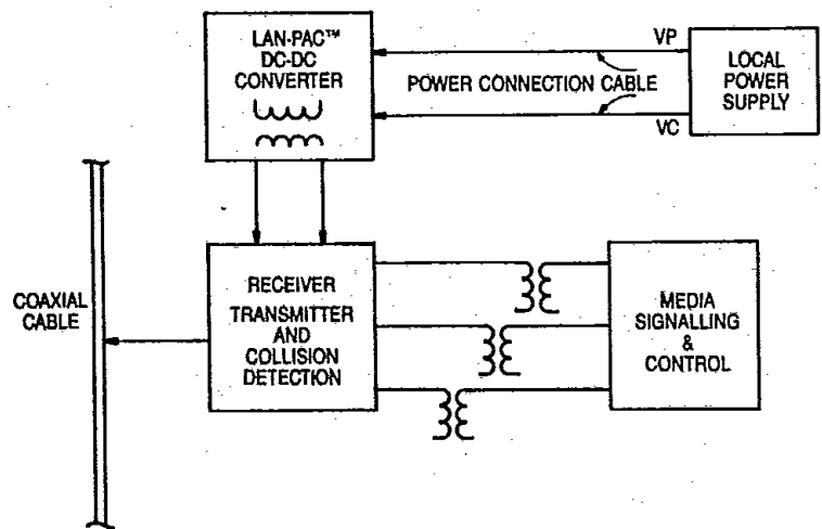
BLOCK DIAGRAM LOCAL AREA NETWORK (LAN)
