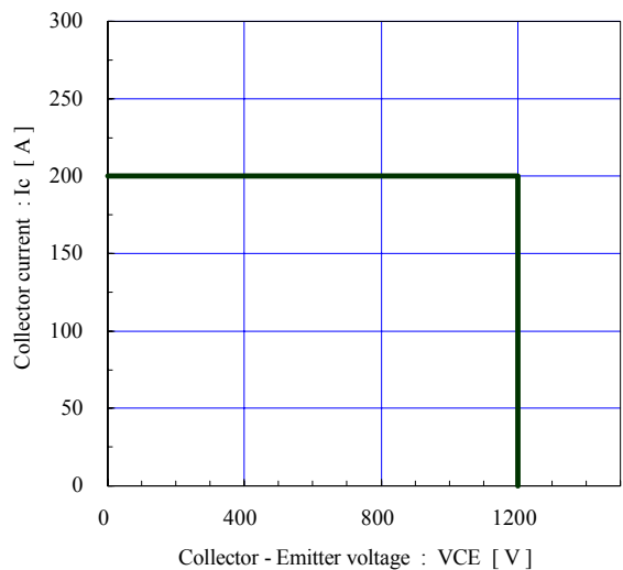
Reverse bias safe operating area (max.) +V_{GE}=15V, -V_{GE} \le 15V, R_g \ge 5.6\Omega, T_j \le 125^\circ C
