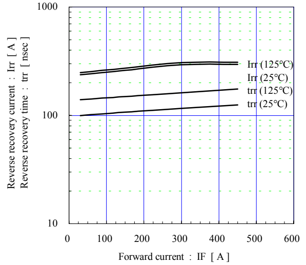
Reverse recovery characteristics (typ.) Vcc=600V, VGE=±15V, Rg=1.1Ω
