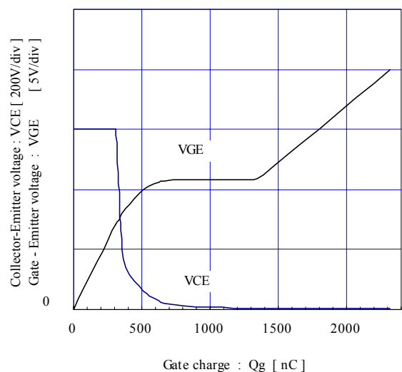
Dynamic Gate charge (typ.) Vcc=600, Ic=450A, Tj= 25°C
