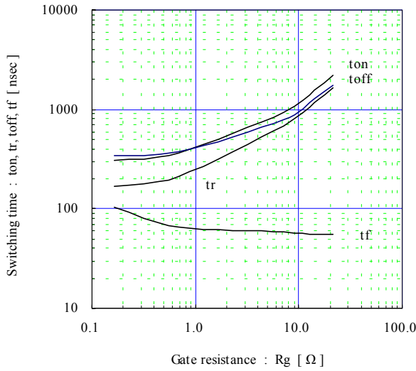
Switching time vs. Gate resistance (typ.) V_{cc}=600V, I_c=450A, V_{GE}=\pm 15V, T_j=25^\circ C
