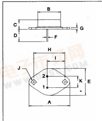
PIN 1. BASE 2. EMITTER COLLECTOR (CASE)
