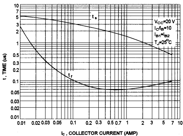
TURN-OFF TIME
