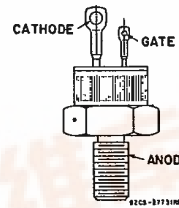
2N5444-46
