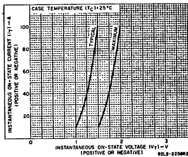
Fig. 5 - On-state current vs. on-state voltage.
