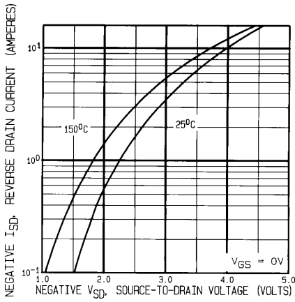
Fig. 7 — Typical Source-to-Drain Diode Forward Voltage
