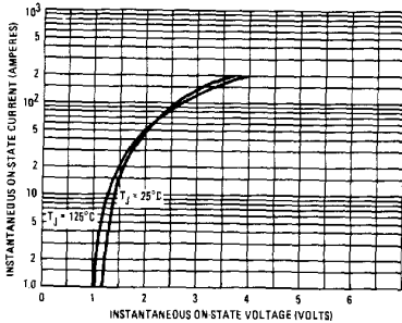
Fig. 14 — Maximum Instantaneous On-State Voltage
