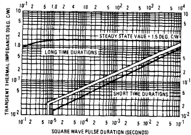
Fig. 15 — Maximum Transient Thermal Resistance
