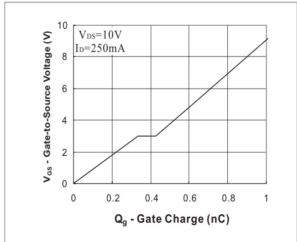
Fig.7 - Gate Charge
