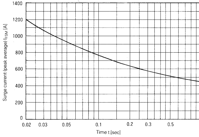
Surge Current
