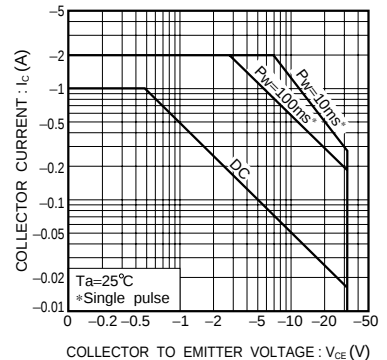
Fig.9 Safe operation area (2SB1132)
