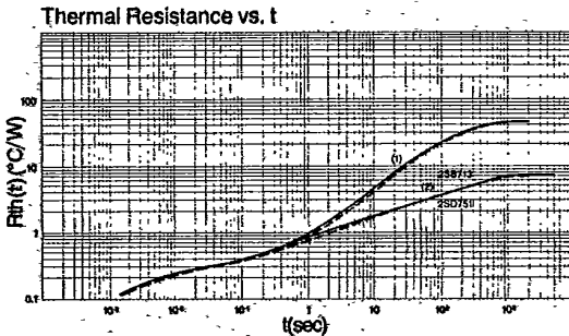
Transient Thermal Resistance Notes: Rth was measured at T_c = 25^\circ\text{C} and under natural convection
