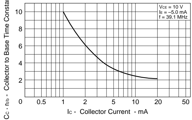
C C · f b'b vs. COLLECTOR CURRENT
