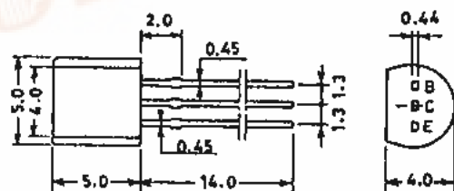
Case Outline 2003A (unit : mm)
