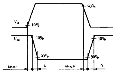
WAVEFORMS
