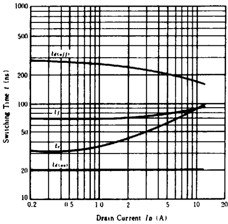
SWITCHING CHARACTERISTICS
