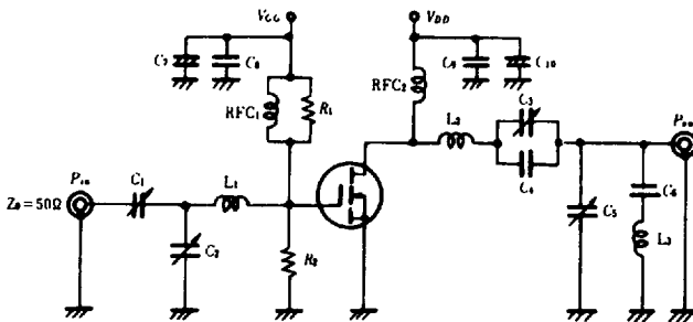
28MHz Pout TEST CIRCUIT
