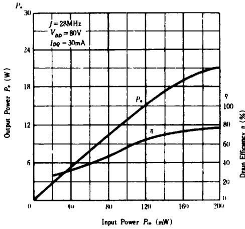
OUTPUT POWER, DRAIN EFFICIENCY VS. INPUT POWER
