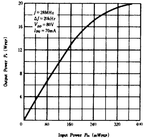
OUTPUT POWER VS. INPUT POWER (2 TONES)
