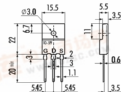
TO-3PF
