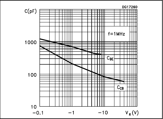
Figure 9. Capacitance
