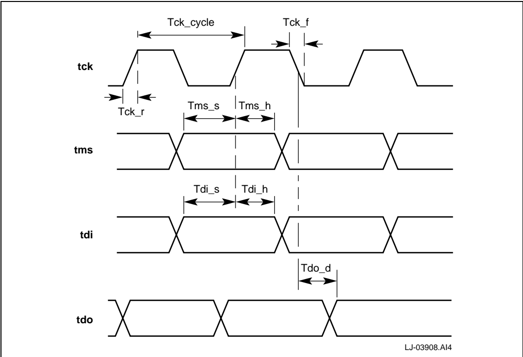
Figure 23. JTAG Boundary-Scan Timing Diagram
