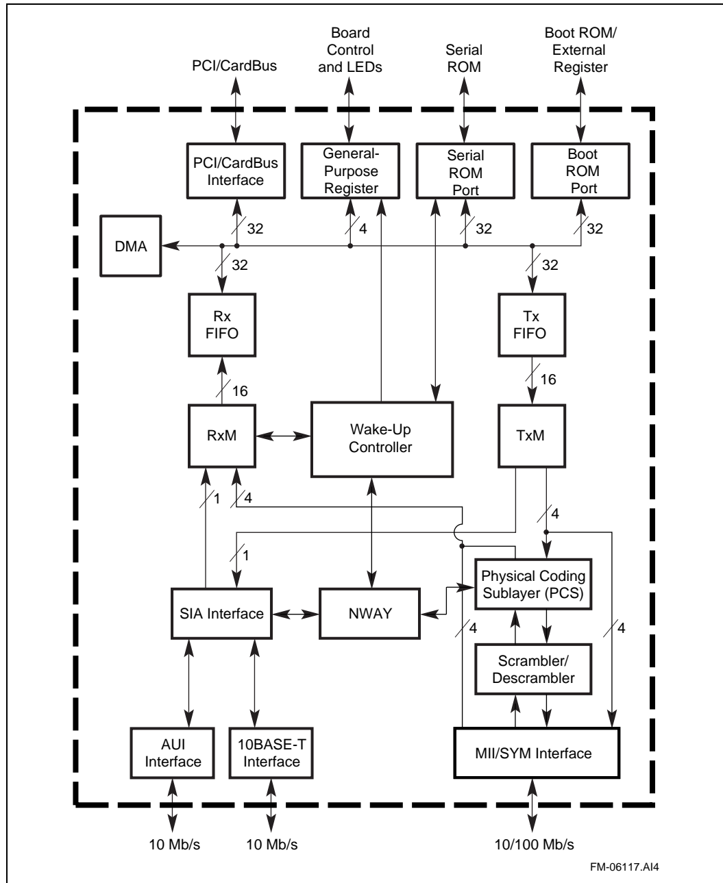
Figure 1. 21143 Block Diagram
