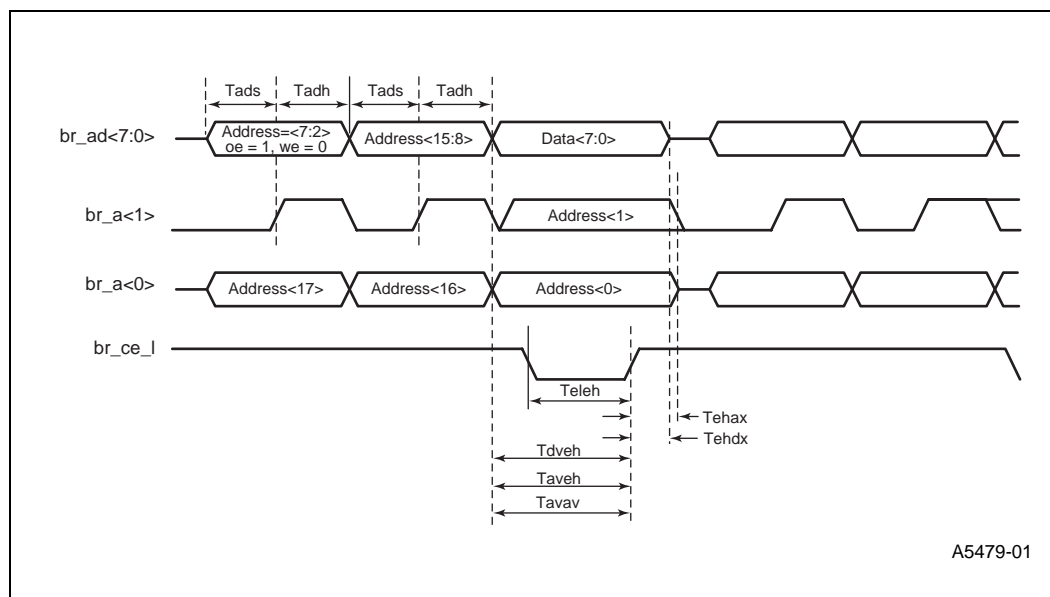
Figure 19 shows the boot ROM write timing characteristics, and Table 34 lists the boot ROM write timing limits.
