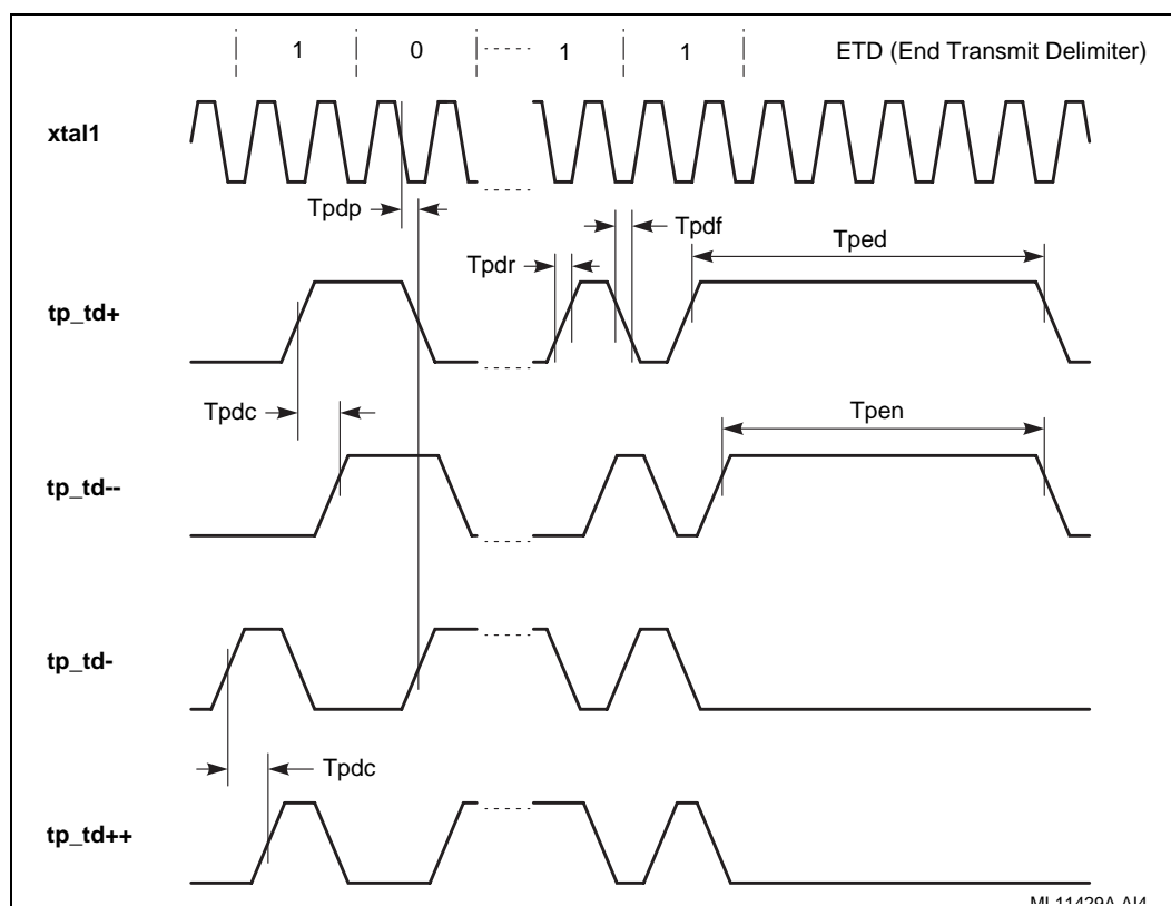
Figure 10. Internal SIA Mode 10BASE-T Interface Timing Diagram—Transmit
