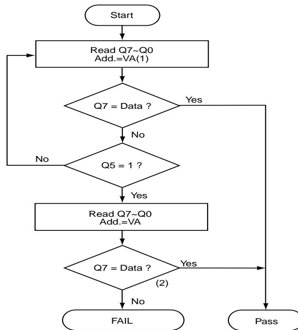
Figure 17. DATA# POLLING ALGORITHM
