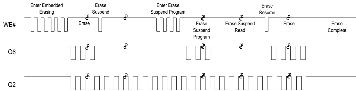
Figure 21. Q6 vs Q2 for Erase and Erase Suspend Operations
