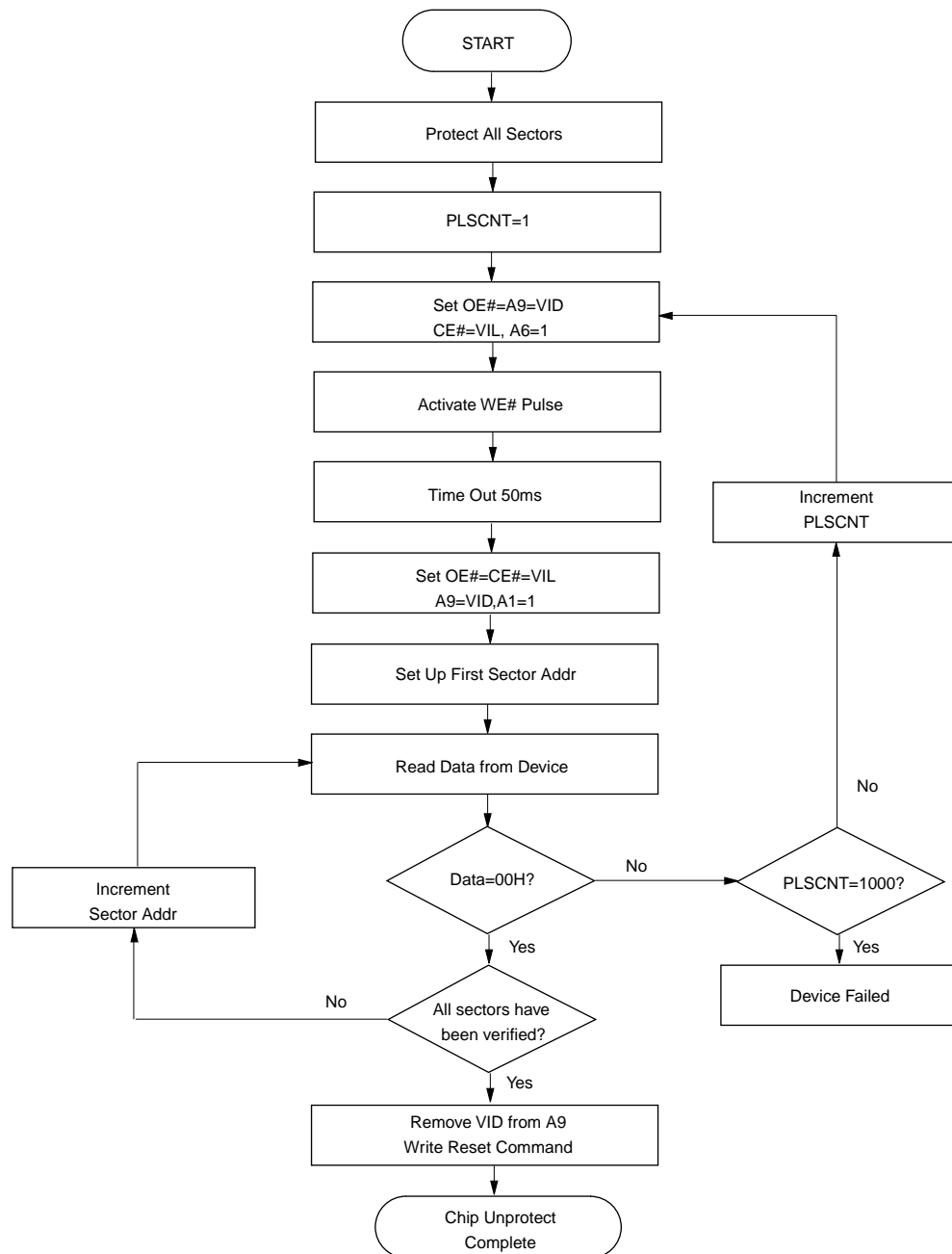
Figure 16. CHIP UNPROTECTED ALGORITHM
