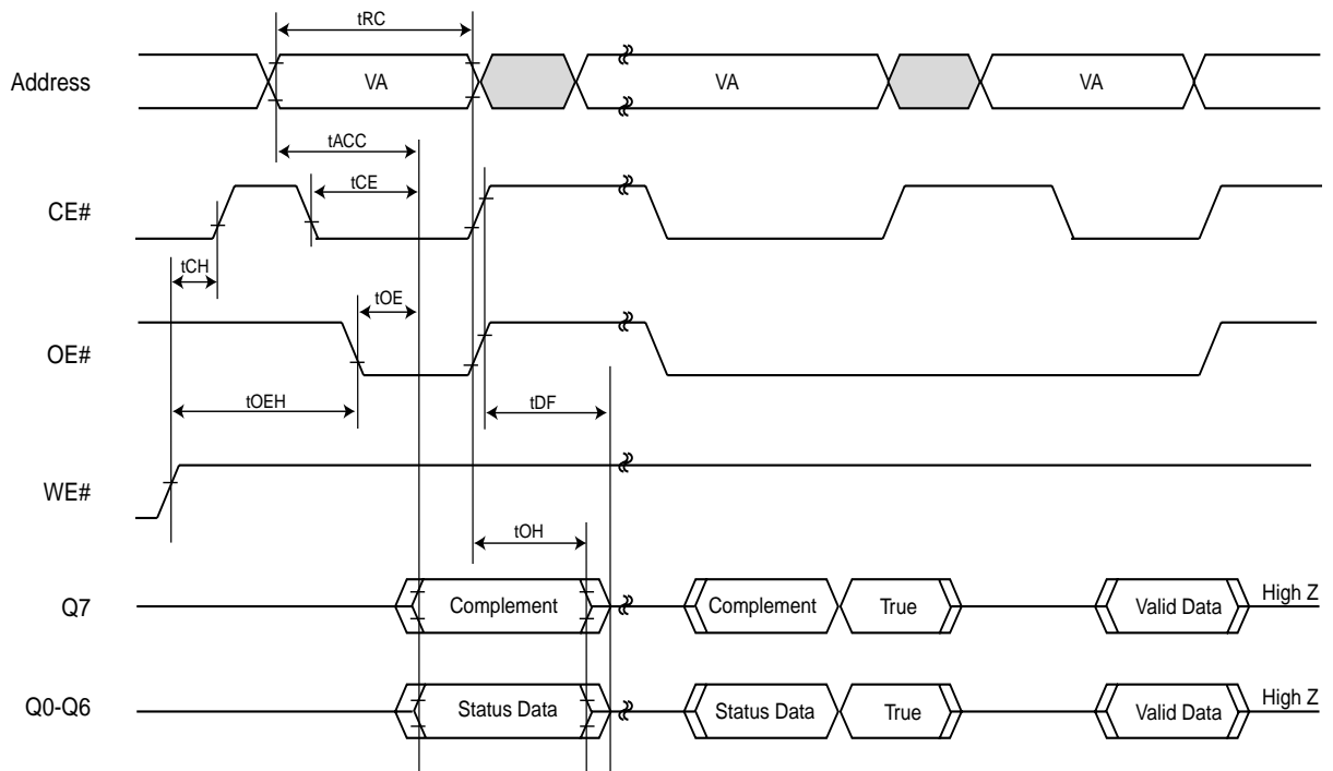
Figure 19. DATA# POLLING TIMINGS (DURING AUTOMATIC ALGORITHMS)
