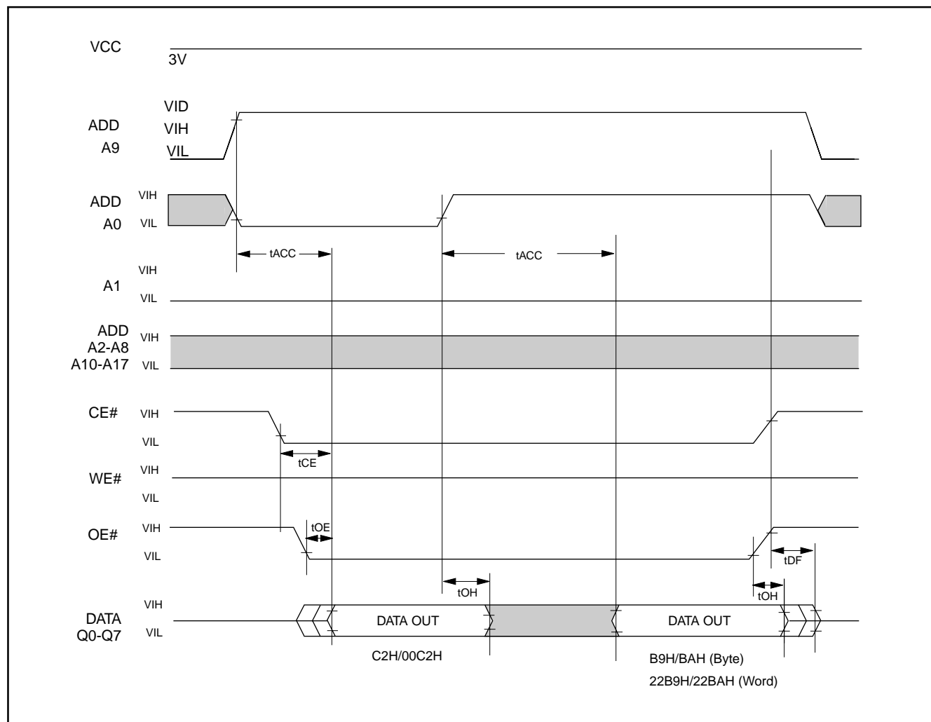
Figure 22. ID CODE READ TIMING WAVEFORM
