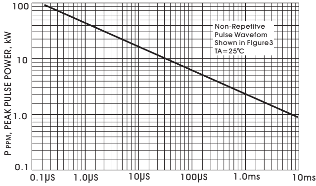
td, PULSE WIDTH, SEC FIGURE 1-PEAK PULSE POWER VS PULSE TIME
