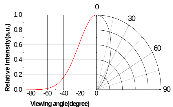
Radiation Characteristics
