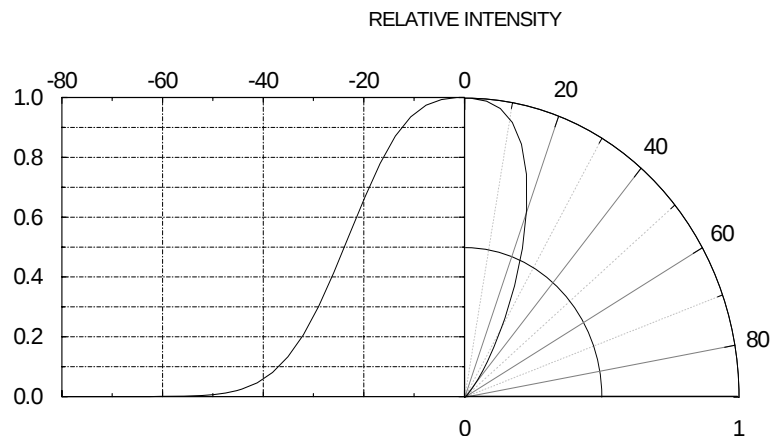
Radiation Characteristics
