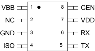
Figure 3. 33290 Pin Connections
