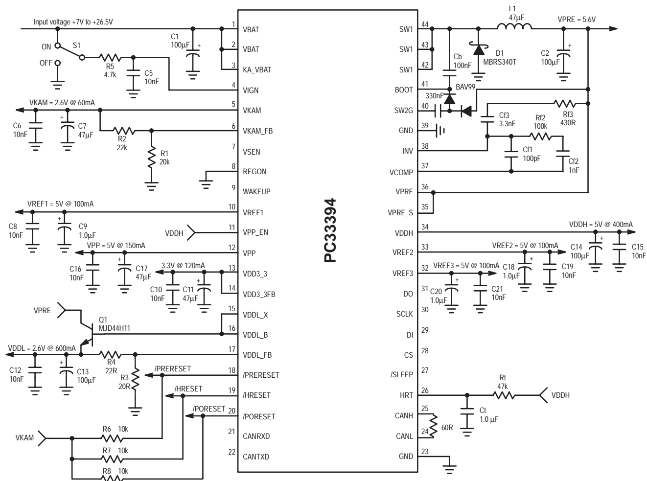
Figure 22. 33394 Buck-Only Application
