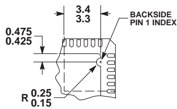
DETAIL M BACKSIDE PIN 1 INDEX OPTION
